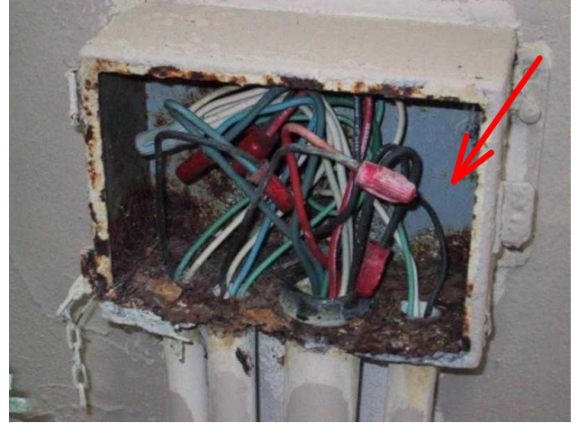
Cover missing and rusted
