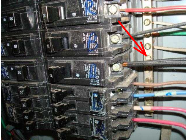
Double tap present
