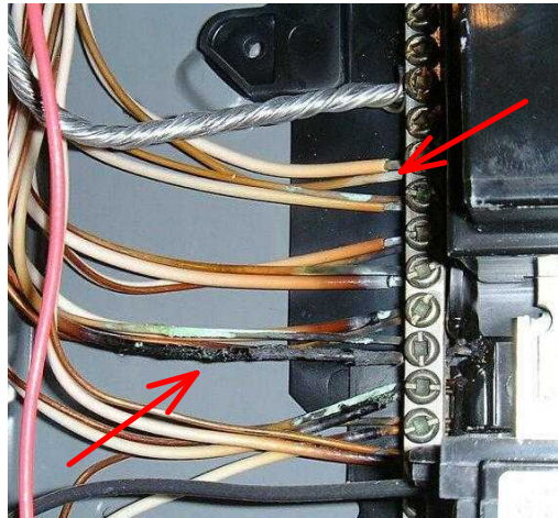
Double taps and burnt wiring
