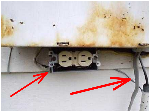
Improper wiring and outlet cover missing
